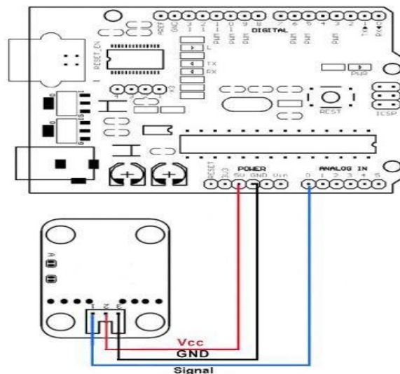
Fig. 6 Interfacing Sensor module with Arduino
