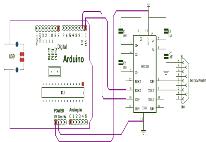
Fig. 8 Arduino interfaced with GSM Module
