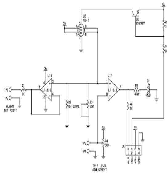
Fig. 5 Connection Diagram of Sensor Module
