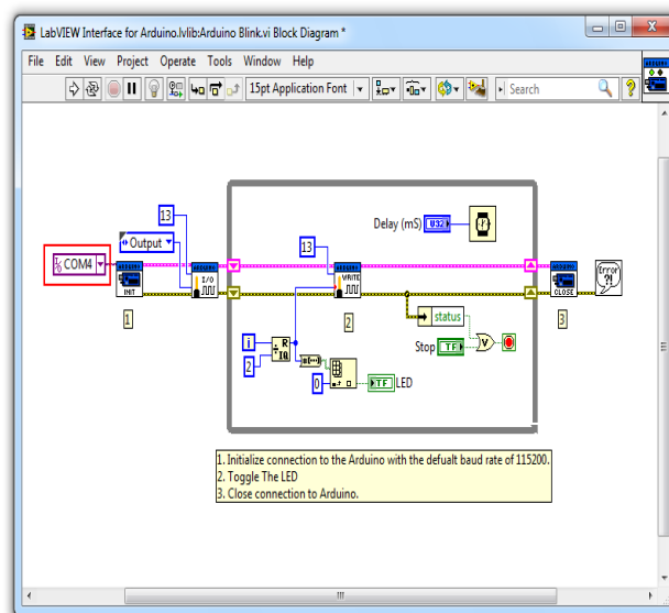
Fig. 11 LabVIEW Block Diagram Linked with Arduino
